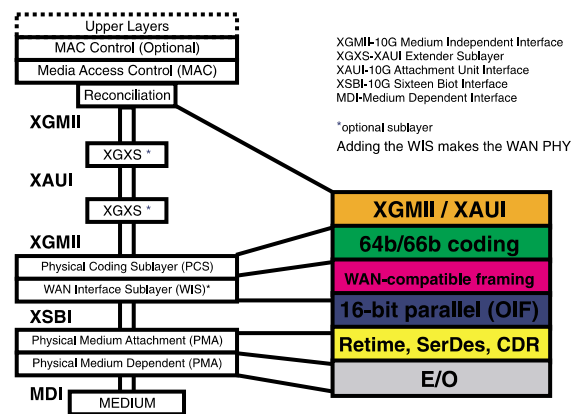
Figure 8. XAUI functions as an extender interface between the MAC and PCS
