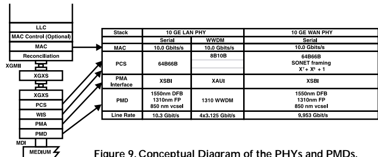
Figure 9. Conceptual Diagram of the PHYs and PMDs.
