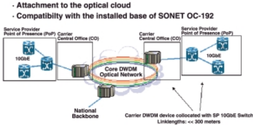
Figure 7. Example of 10 Gigabit Ethernet in WAN applications
