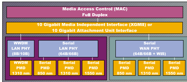
Figure 2. The architectural components of the 802.3ae standard
