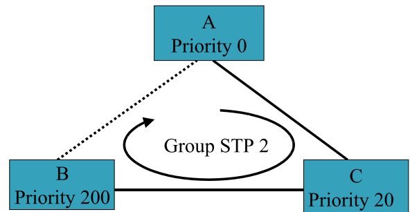
Figure – 8(b): Provisions for Group STP2.
