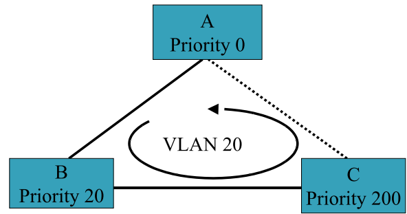
Figure – 7(b): Provisions for VLAN 20
