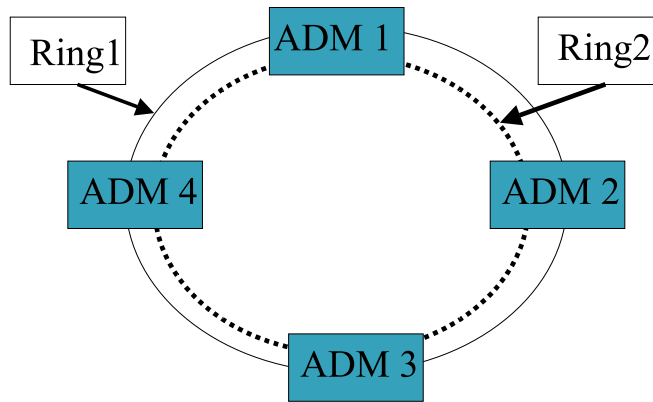
Figure – 3(b): Bi-directional Line Switched Ring.
