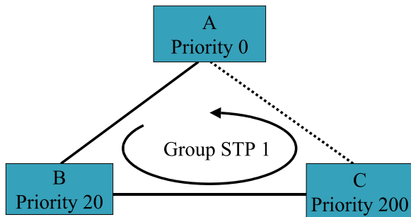
Figure – 8(a): Provisions for Group STP1.
